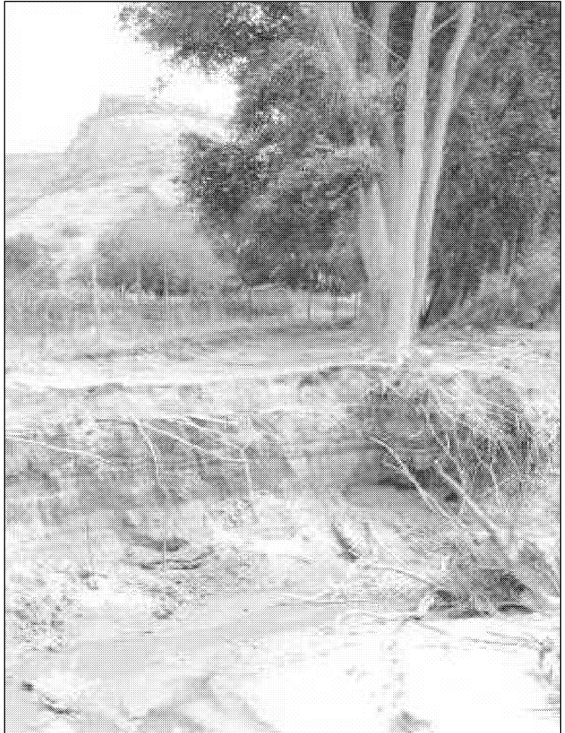
Figure 12. Complete road wash out on Tsaile Creek Watershed. 96-0025WPF
