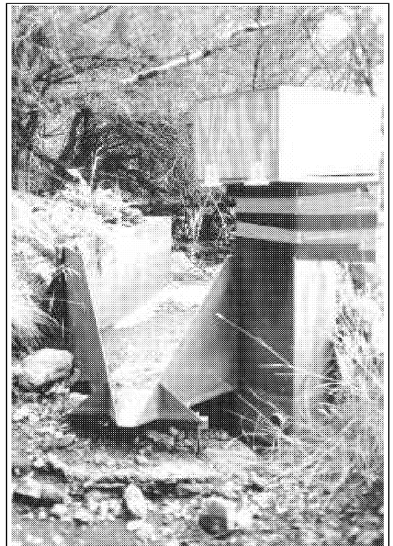
Figure 10. Flume installed to measure stream flow at Hart Prairie. 95-005WPF.
