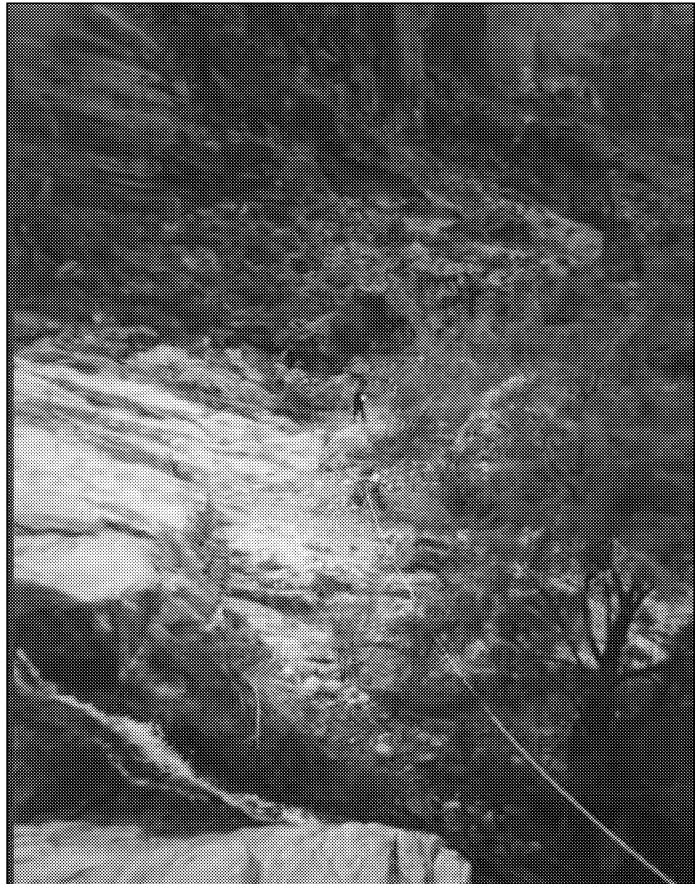
Figure 19. Establishing sampling transects along a tributary of the Colorado River. 99-075WPF
